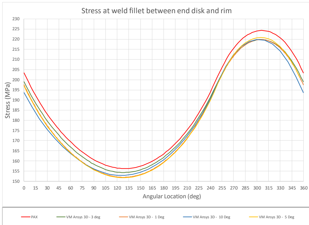
Figure 28. Von Mises stress at fillet weld between end disk and rim
