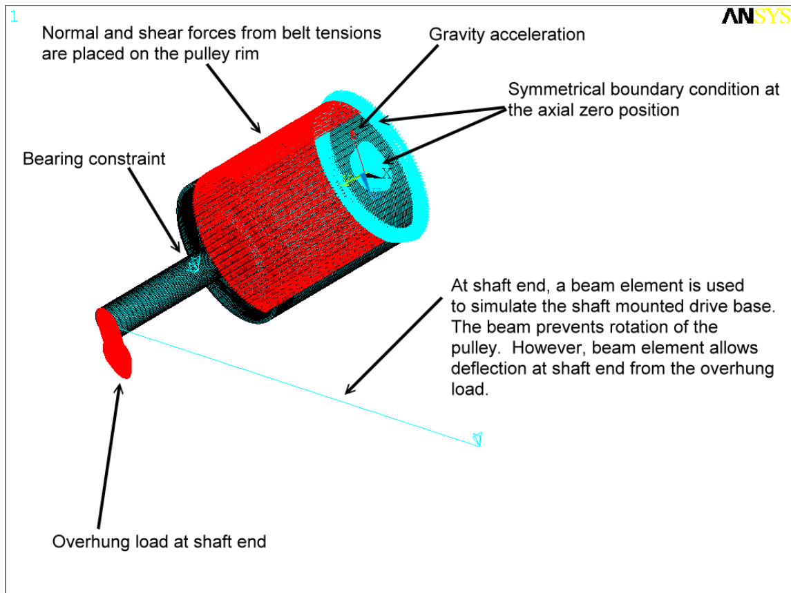
Figure 2. Boundary conditions of symmetrical drive pulley
