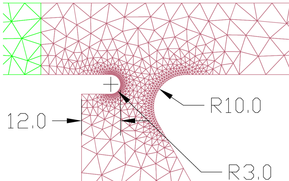
Figure 25. Zoom into weld geometry
