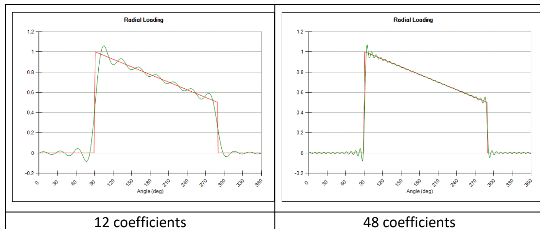
Figure 5. Fourier series fit of radial square wave with 12 and 48 coefficients
