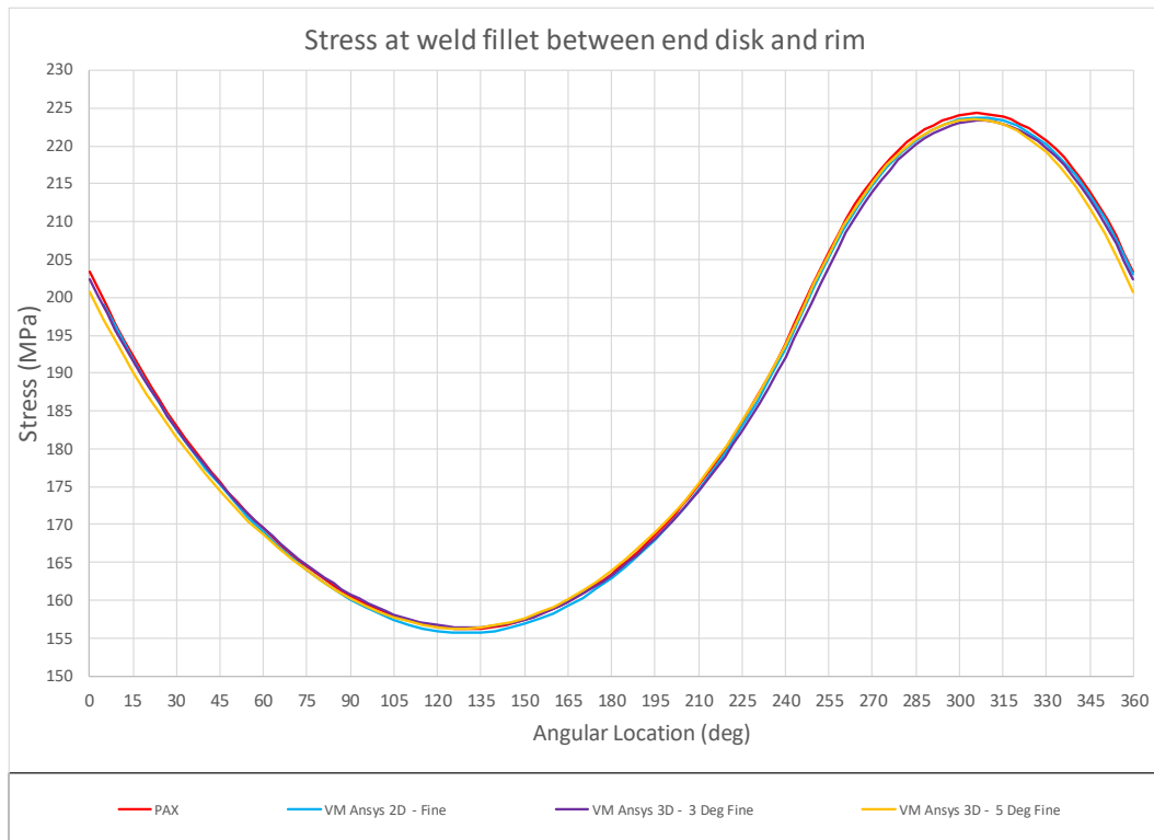
Figure 30. Von Mises stress at fillet weld between end disk and rim with refined 3D model
