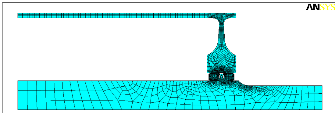
Figure 8. ANSYS 2D Element Plot of Pulley
