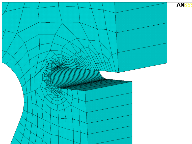
Figure 29. Refined 3D elements at weld fillet (5 degree element rotation angle)
