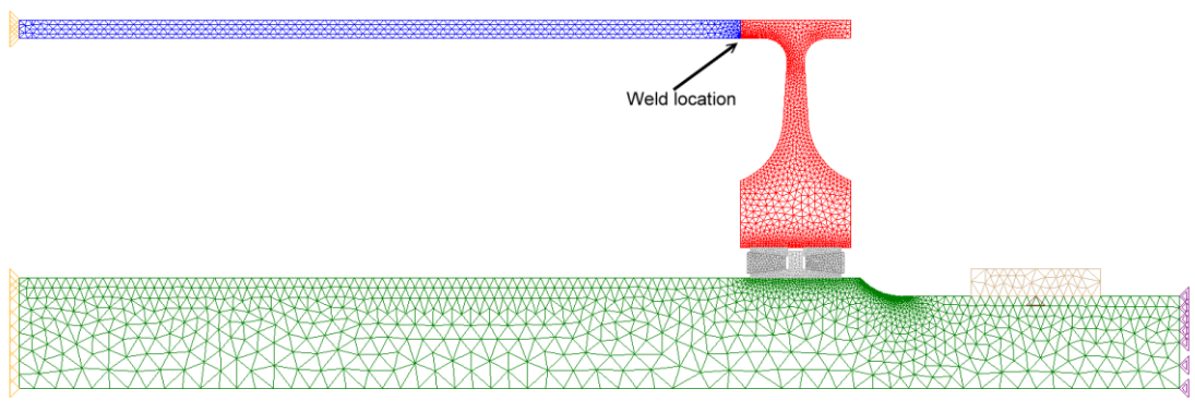
Figure 7. PAX Element Plot of Pulley
