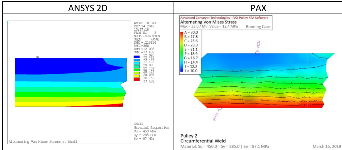
Figure 12. Alternating stress at inside edge at the weld location between rim and end disk
