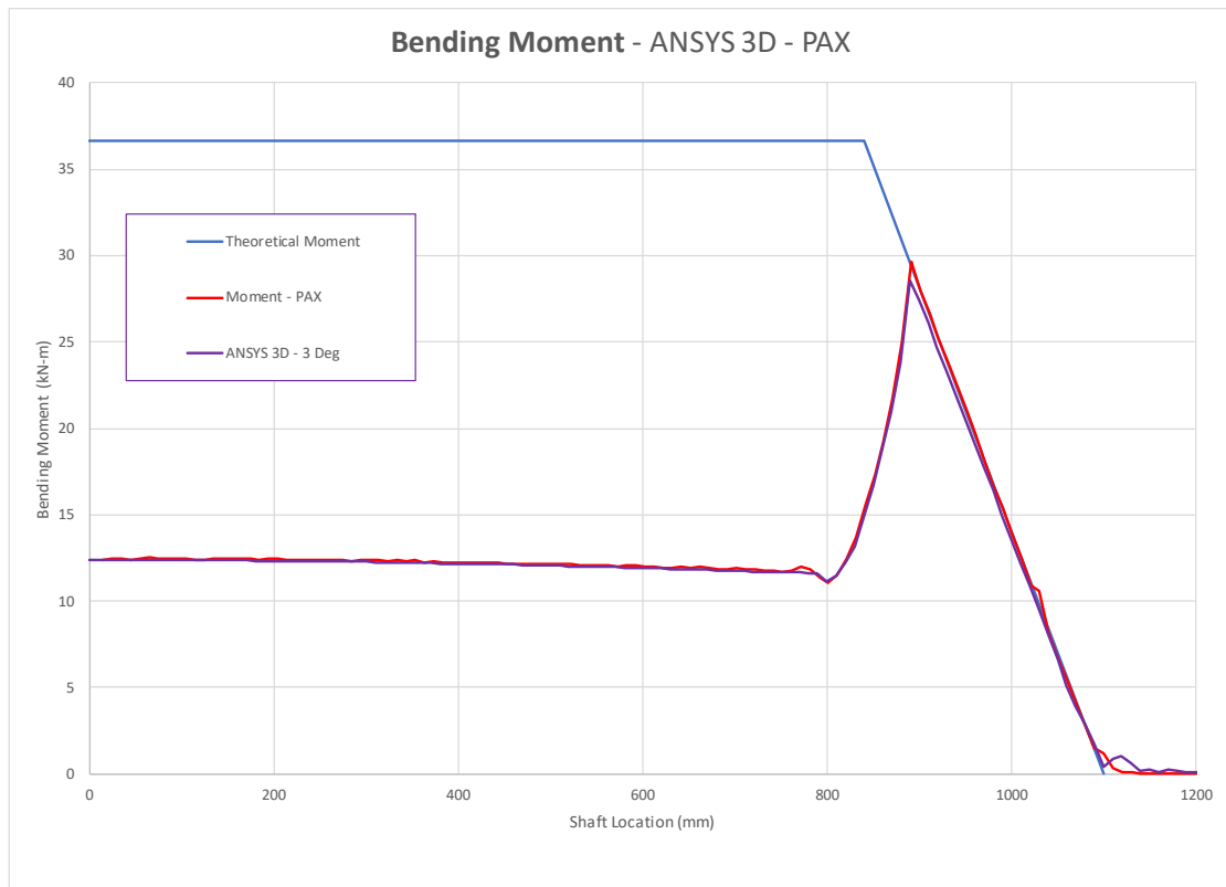
Figure 19. Bending moment in shaft
