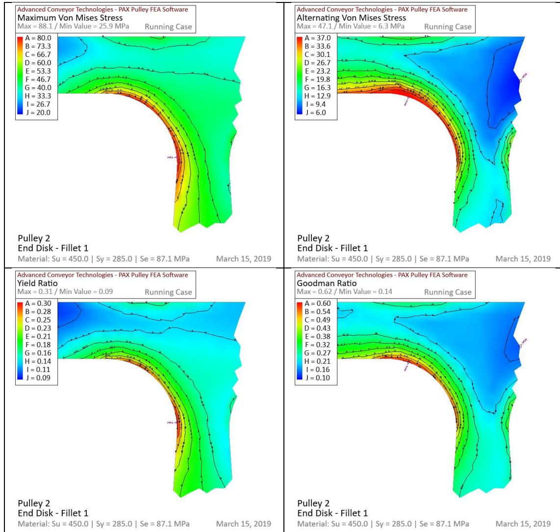
Figure 23. Contour plots of fatigue stresses and failure ratios based on full 360° rotation (PAX)
