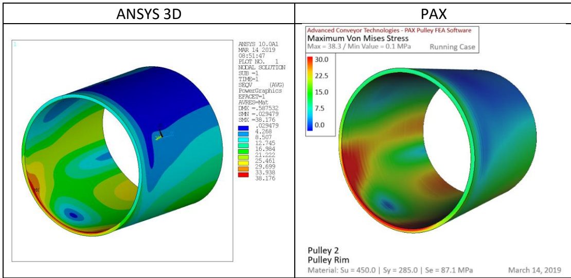
Figure 11. Stress at inside edge at the weld location between rim and end disk
