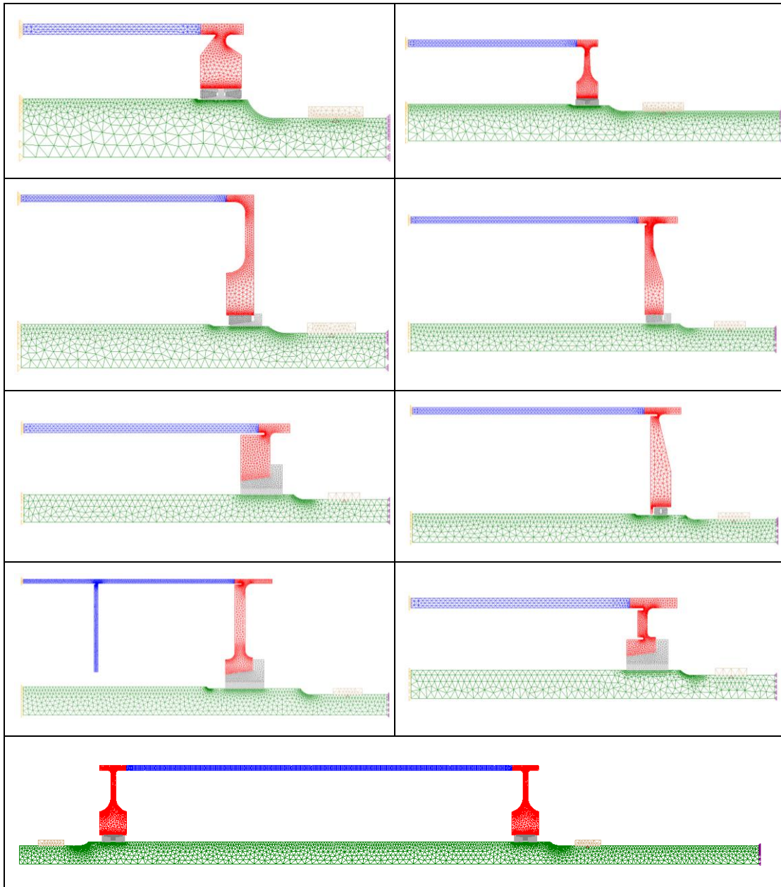
Figure 20. Various pulley geometries analysed using full 3D and 2D axis-symmetric elements
