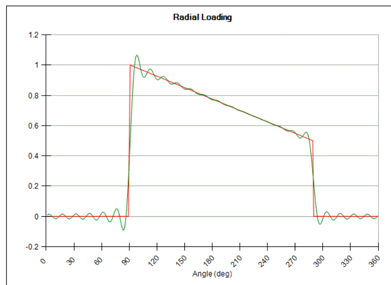
Figure 4. Fourier series fit of radial square wave with 24 coefficients
