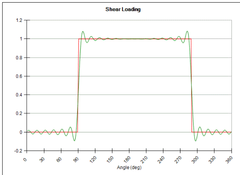
Figure 6. Shear Pressure Fourier Series (24 coefficients)
