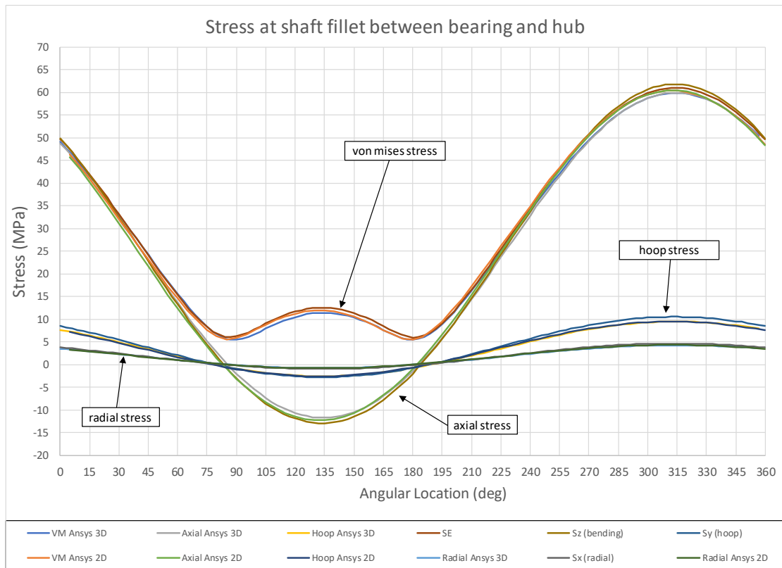
Figure 17. Stress at shaft fillet between bearing and hub
