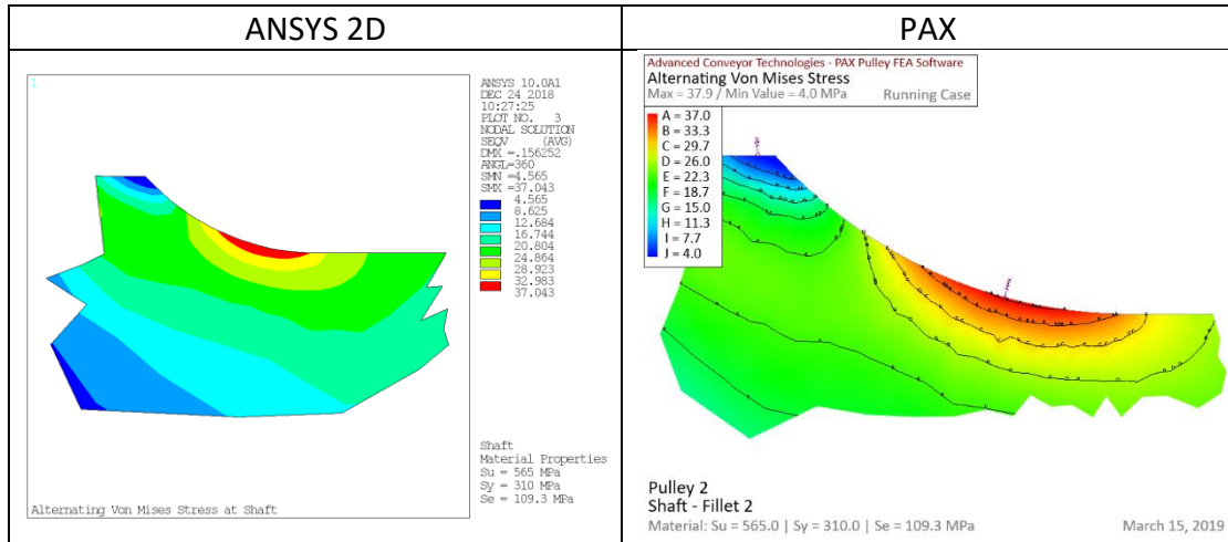
Figure 16. Alternating stress at bearing fillet in shaft
