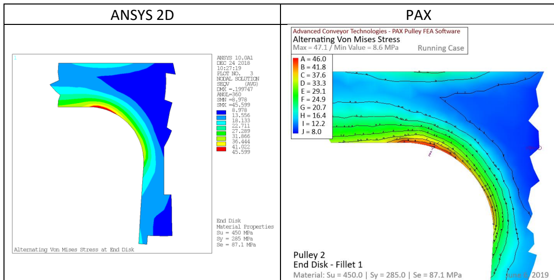
Figure 13 Alternating stress at inside edge at the weld location between rim and end disk
