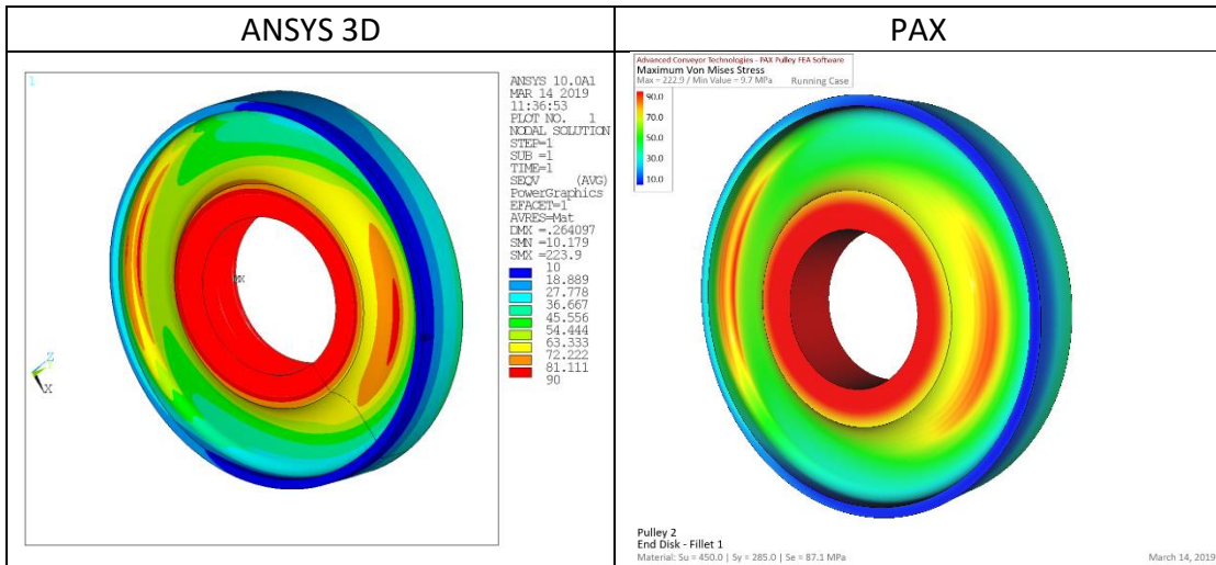
Figure 15. Von mises stress in end disk
