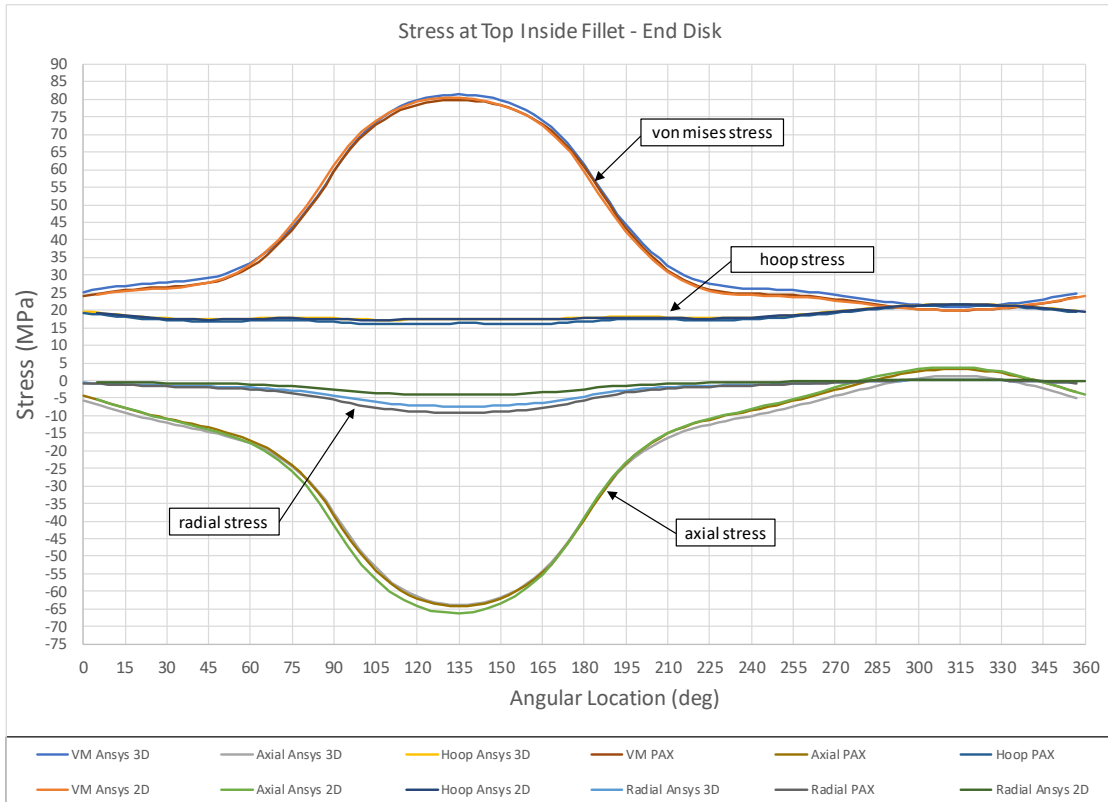
Figure 14. Stress at top inside fillet in the end disk
