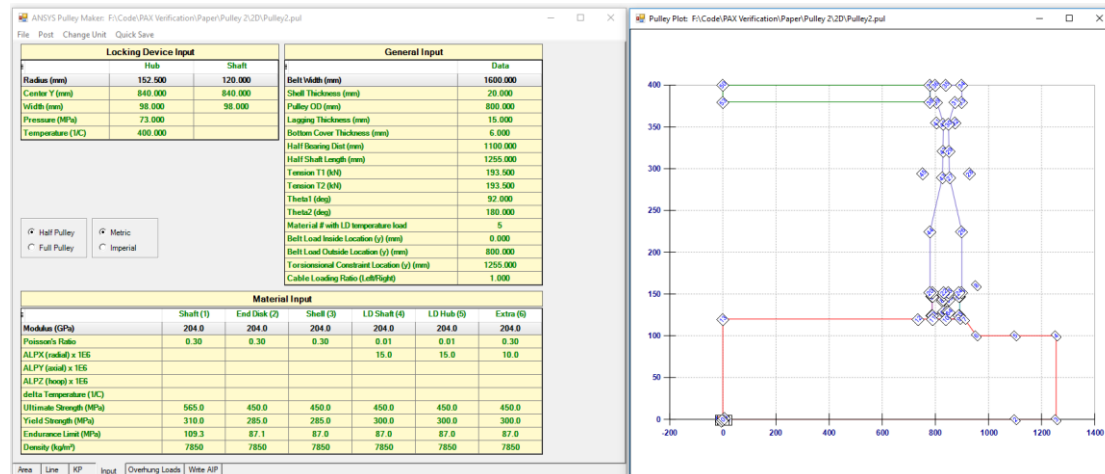
Figure 21. AC-Tek’s interface of ANSYS Pulley Maker
