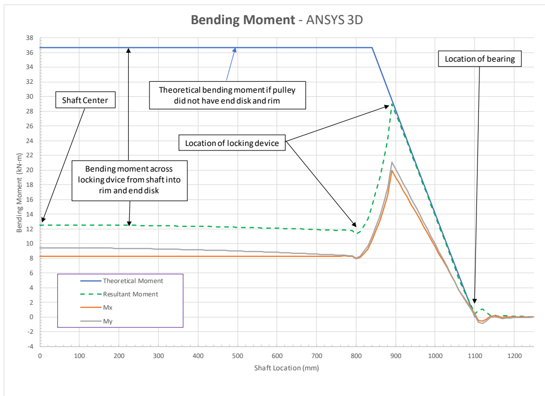
Figure 3. Bending moment calculation from finite element model
