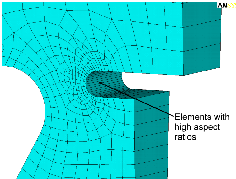
Figure 27. 3D elements at weld fillet (5 degree element rotation angle)
