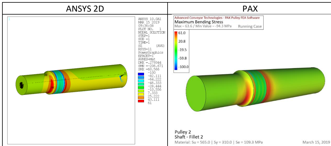
Figure 18. Axial (bending) stress in shaft
