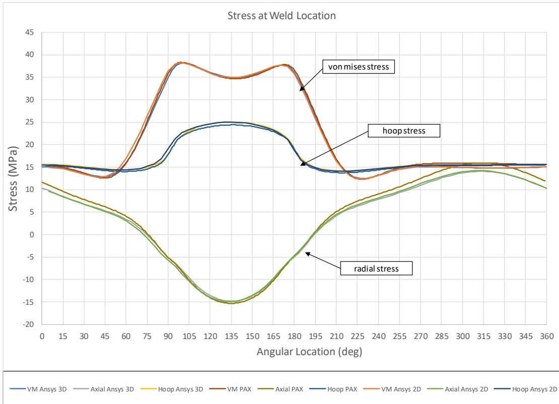
Figure 10. Stress at inside edge at the weld location between rim and end disk
