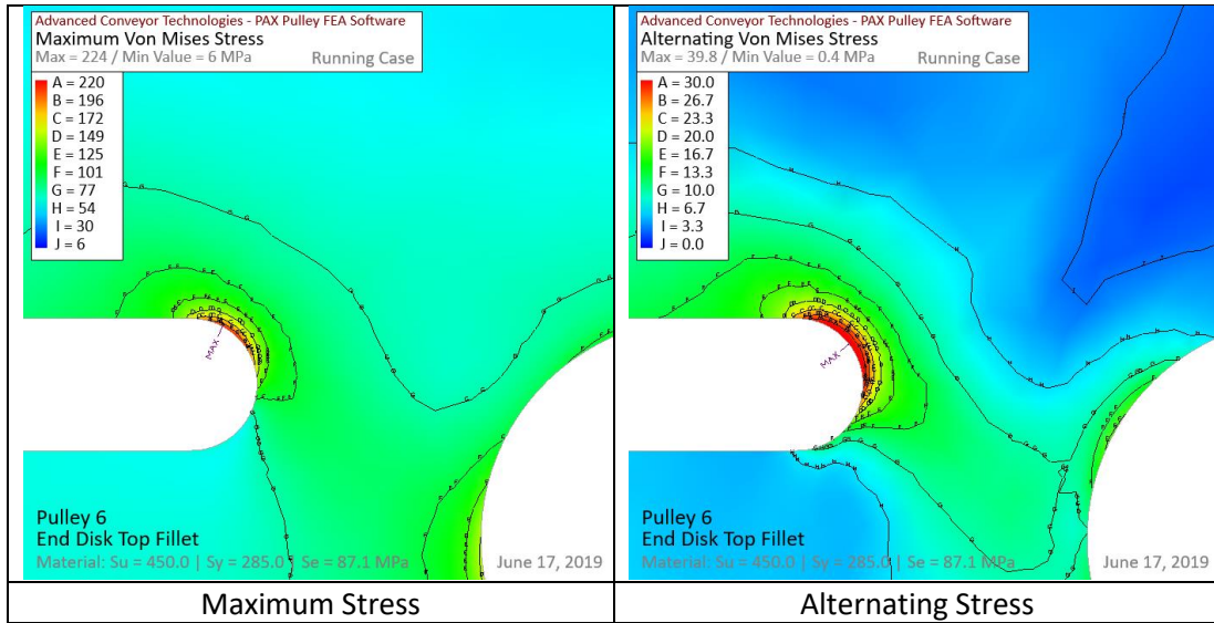
Figure 26. Alternating von mises stress in the weld (PAX)
